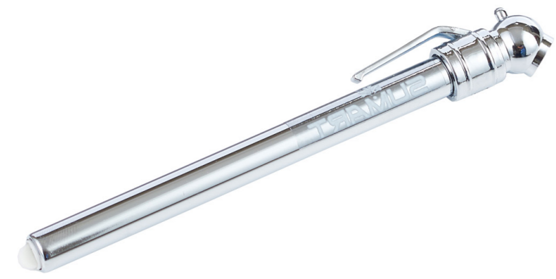
TPG02 | TIRE PRESSURE GAUGE + MEASURING RANGE : 5 - 50 (PSI)
